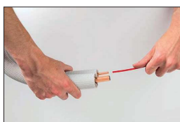
STEP 1 INSERT THE FLEXIBLE BENDER OF THE RIGHT DIAMETER INTO THE COPPER TUBE.
