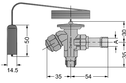
Figure: Flare × solder
