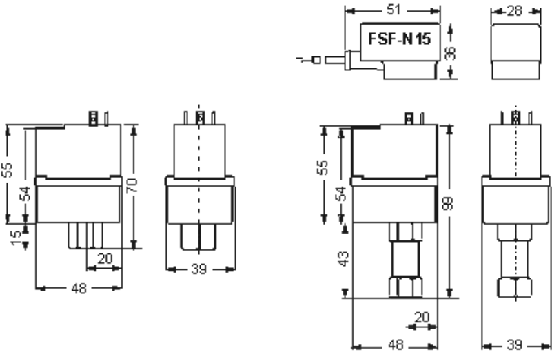
FSY / FSM-41S FSY / FSM-42S FSY / FSM-43S
